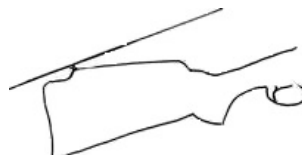
Crosse Monte-Carlo
